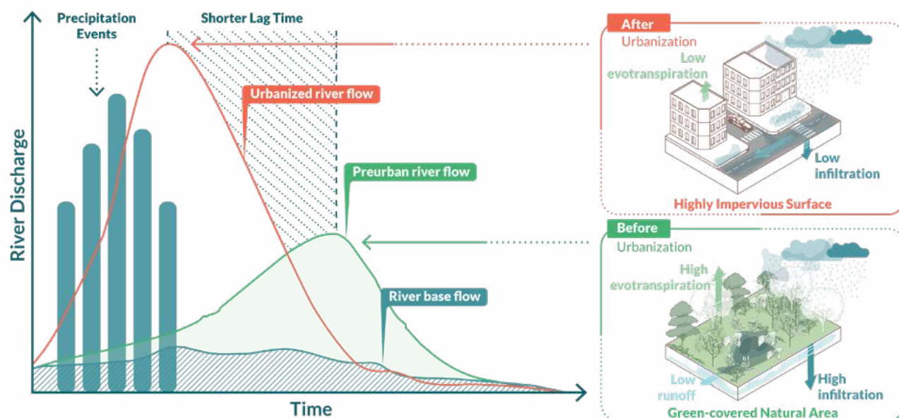
Figure 5.4: Effects of Urbanization and Flood Control Measures on Flow Velocity
