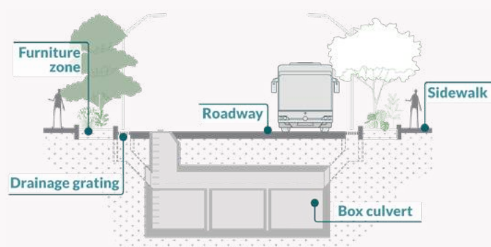
Figure B4.1.2 Box Culvert Section and Public Works
