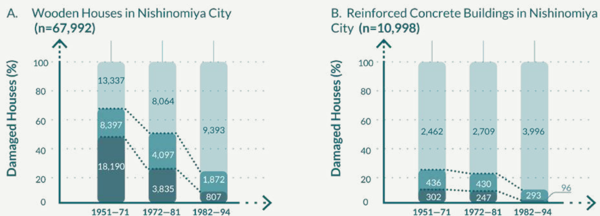
Figure B6.2.2: Damage to Building Structures in the Great Hanshin-Awaji Earthquake by Period of Construction
