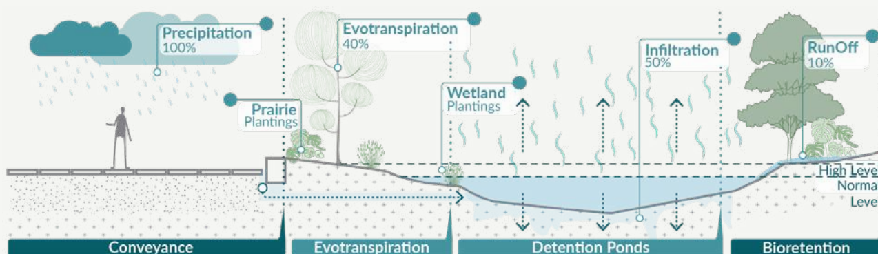
Figure B5.1.1: Reduction of Flooding by Retaining and Gradually Releasing Surplus Water through Quality Control Mechanisms
