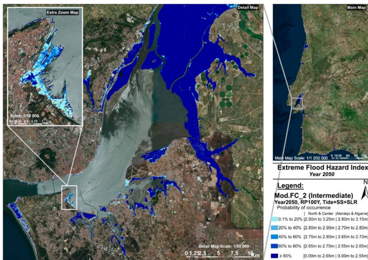
Figure 5.5.1: Example of Portuguese Coastal Flooding Extreme Scenarios for 2050 Sea-Level Rise and 100-Year Return Period
