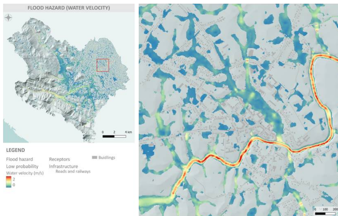
Figure 5.2.1: Examples of a Flash Flood Hazard Map and a Flow Velocity Hazard Map, Croatia
