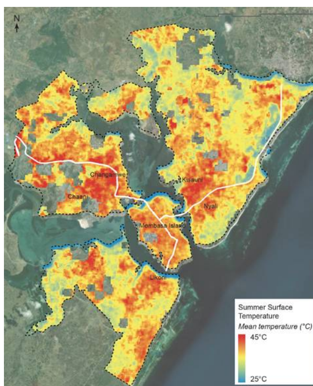
Figure 7.1.1: Example of Summer Surface Temperature Map for Mombasa, Kenya
