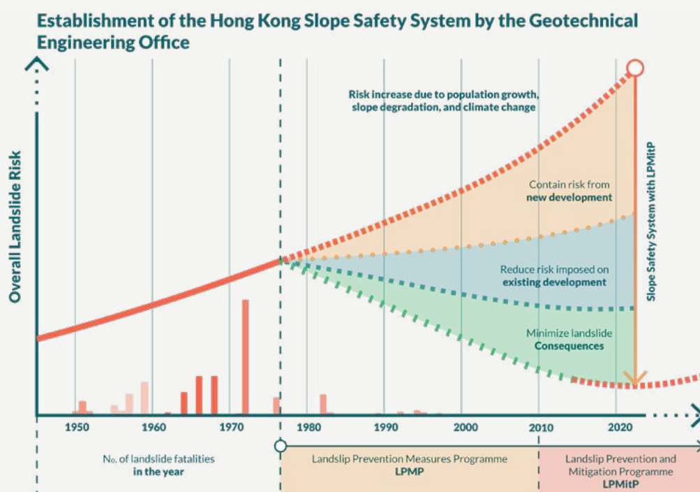
Figure B6.1.1: Impact of Landslide Risk Reduction Strategies in Hong Kong
