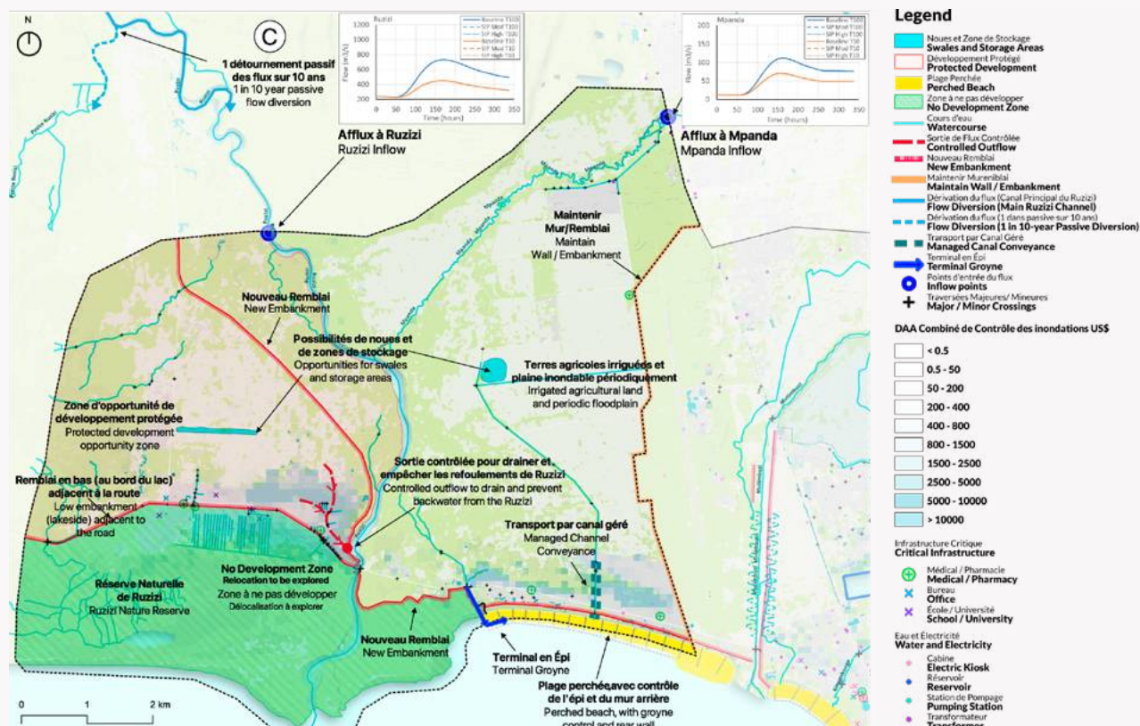
Figure B3.1.1: Hazard and Risk Modeling and Strategic Plan for Flood Risk Management in Ruzizi Catchment
