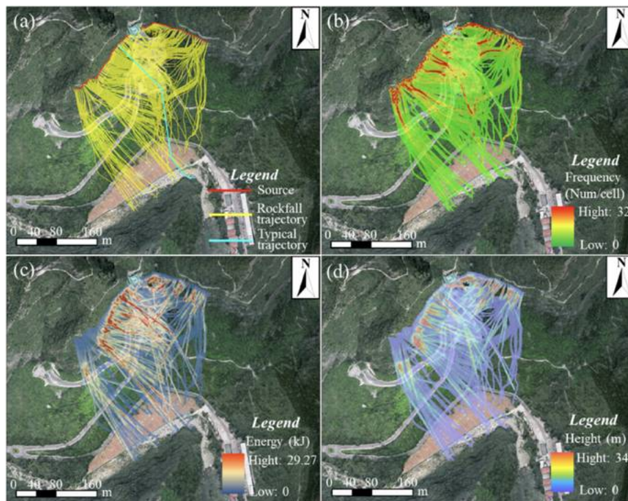
Figure 6.3.1: Example of Rockfall Hazard Assessment – Spatial Distribution of Disaster-Causing Factors in the Scenic Spot of Sky City, China
