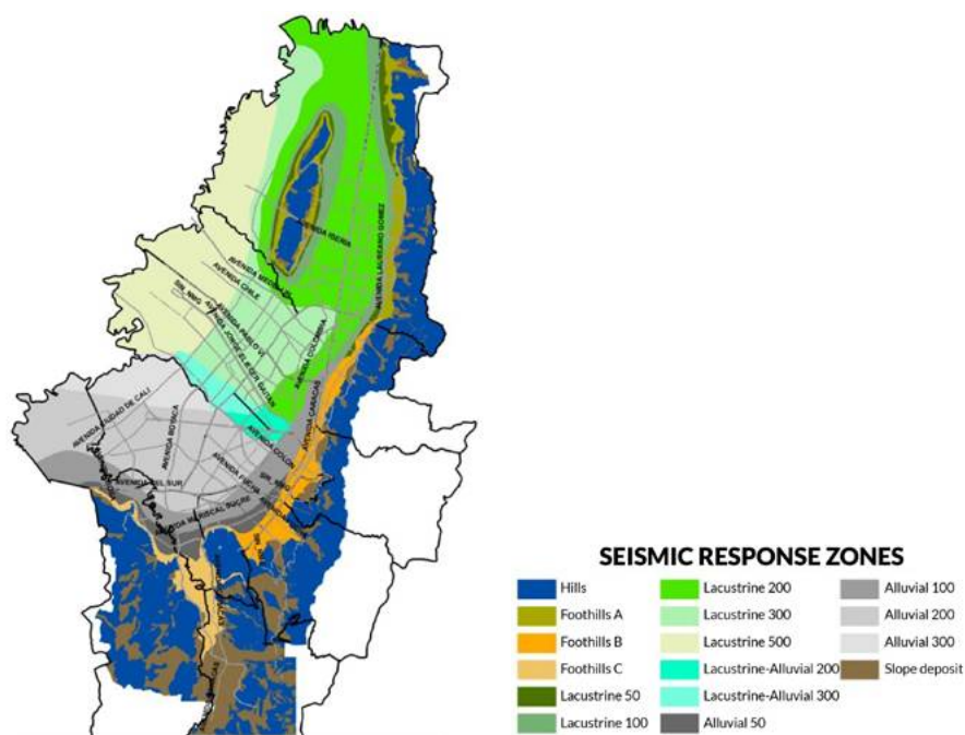
Figure 6.4.1: Seismic Microzonation in Bogota, Colombia
