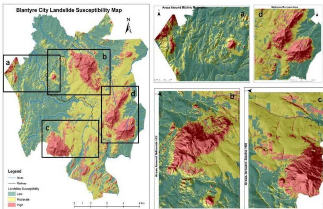
Figure 6.1.1: Example of a Landslide Susceptibility Map for Blantyre City, Malawi
