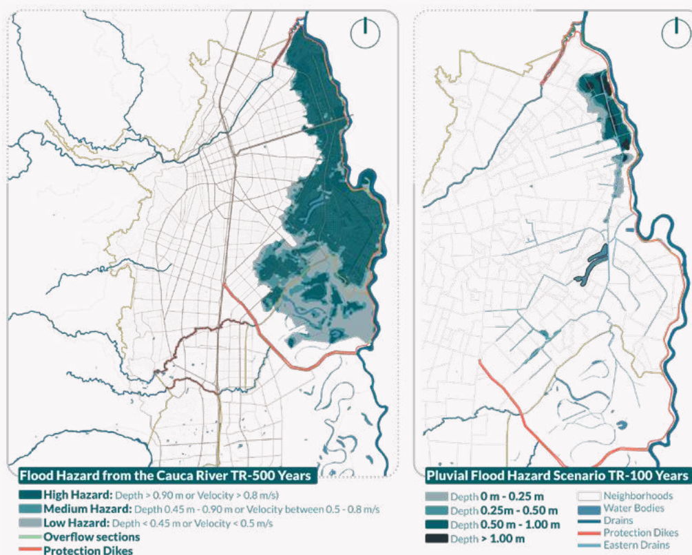
Figure B3.2.1: Fluvial and Pluvial Hazard Maps
