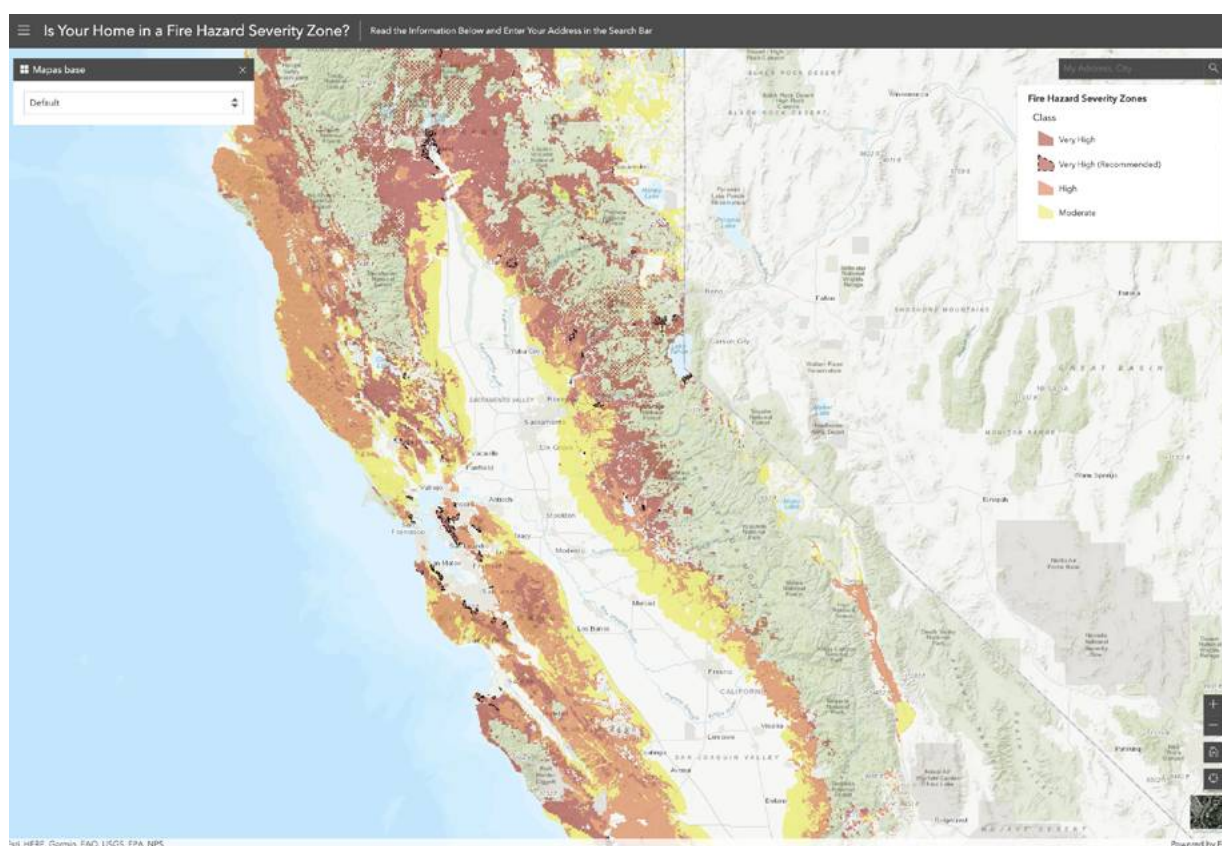
Figure 7.3.1: Example of Fire Hazard Severity Zones for California State
