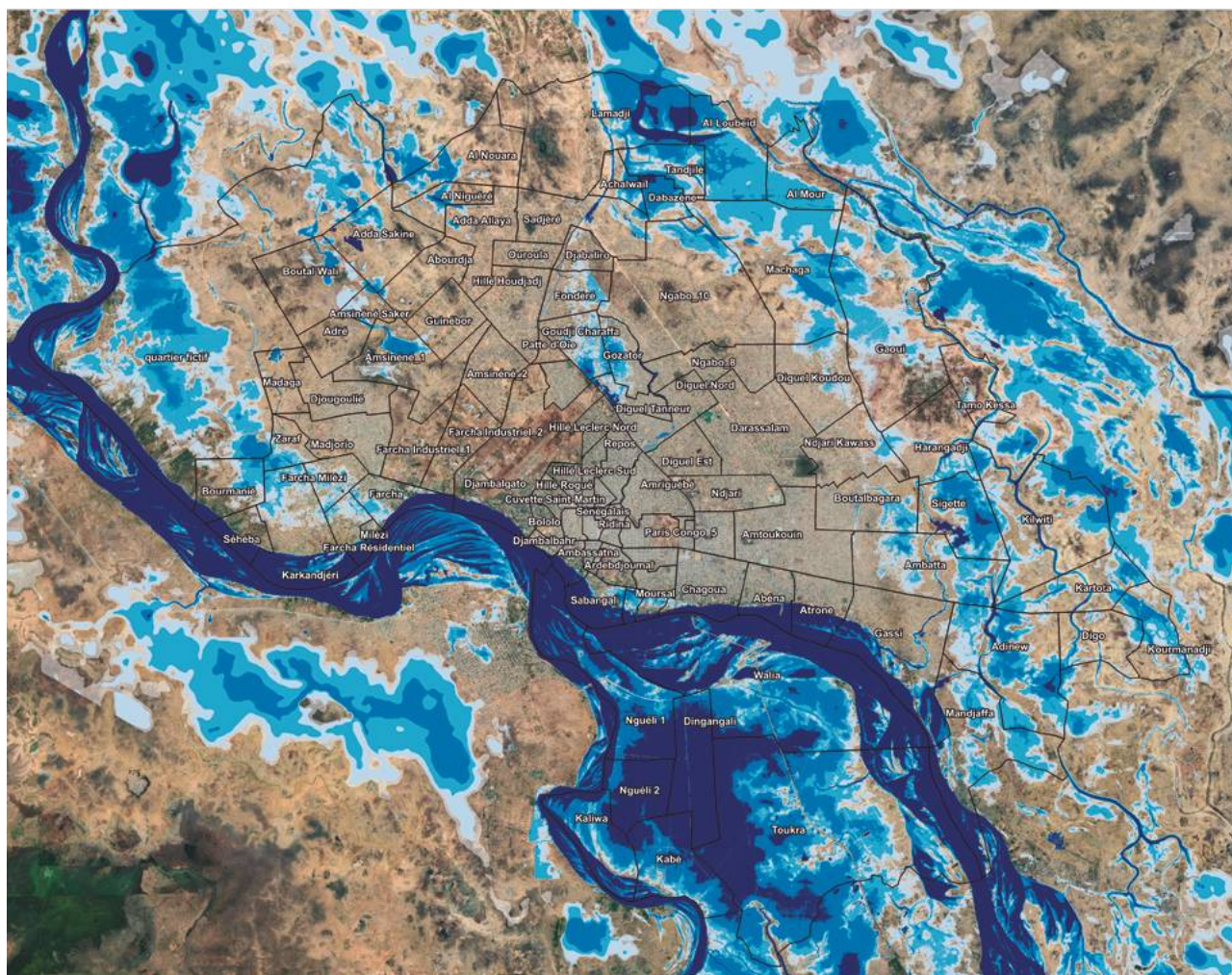
Figure 5.4.1: A River Flood Hazard Map of the Chari and Logone Rivers in N'djamena, Chad, for a 100-Year Flood (2023 Status)
