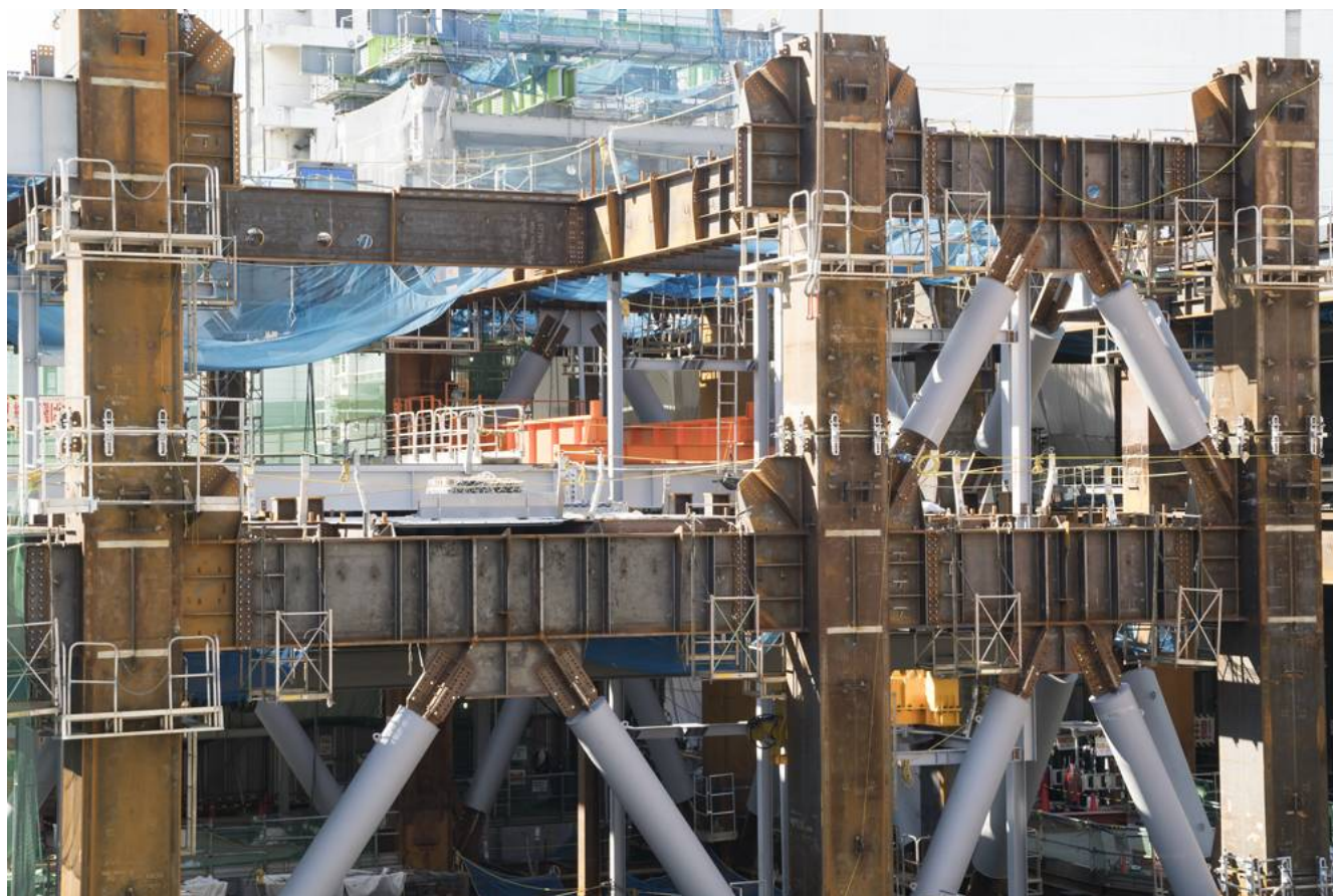
Photo 4.1: Construction of Earthquake-resistant Steel Structure in Tokyo
