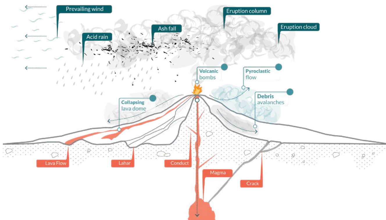
Figure 6.3: An Illustration of Common Proximal Volcanic Hazards
