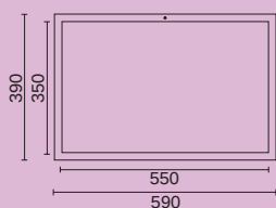
MARCO IPF 39 PUERTA INOXIDABLE REF. M39PI
