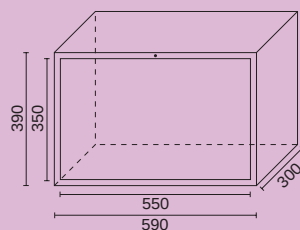
MARCO IPF 39 PUERTA INOXIDABLE REF. M39PI
