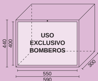
COFRE IPF 41 PUERTA PINTADA REF. C41PP
