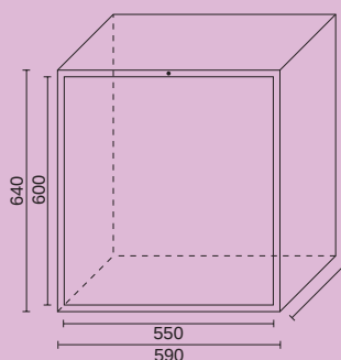
COFRE IPF 40 PUERTA INOXIDABLE REF. C40PI
