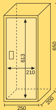
PUERTA CIEGA EXT 6-12 kg REF. EXTPM6
