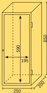
PUERTA EXT 6-12 kg REF. EXTPC6
