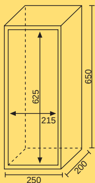
GUÍA EXT.6-12 kg REF. EXT6E
