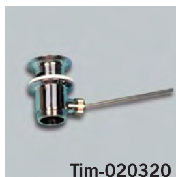
Click clack valve set material: Chrome plated brass high polished valve diameter: 63 mm 1/4"
