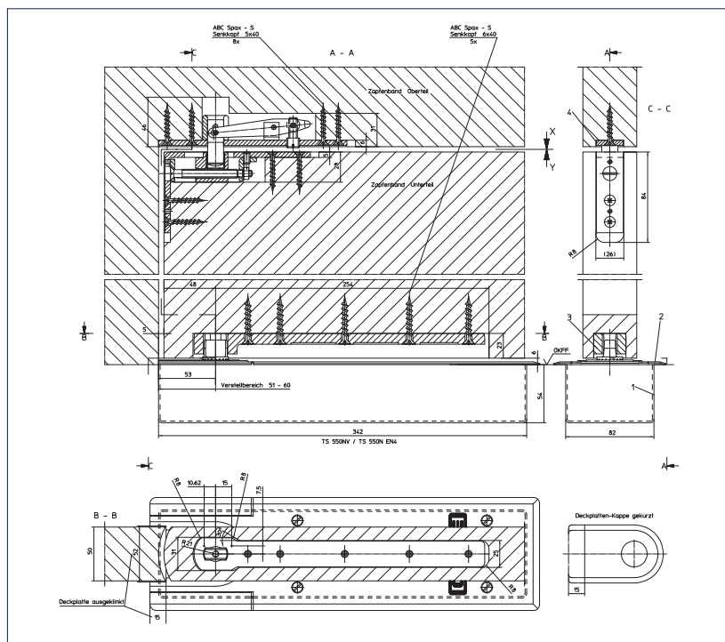
Fig. 30-2 · Standard installation of GEZE TS 550 NV to a double action door
