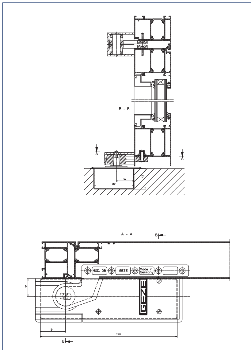
Fig. 28-1 · Standard installation of GEZE TS 500 NV to a single action door
