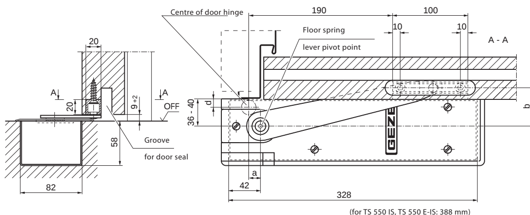
Fig. 34-2 · Installation example: floor spring with lever and guide rail (concealed) to a flush timber door
