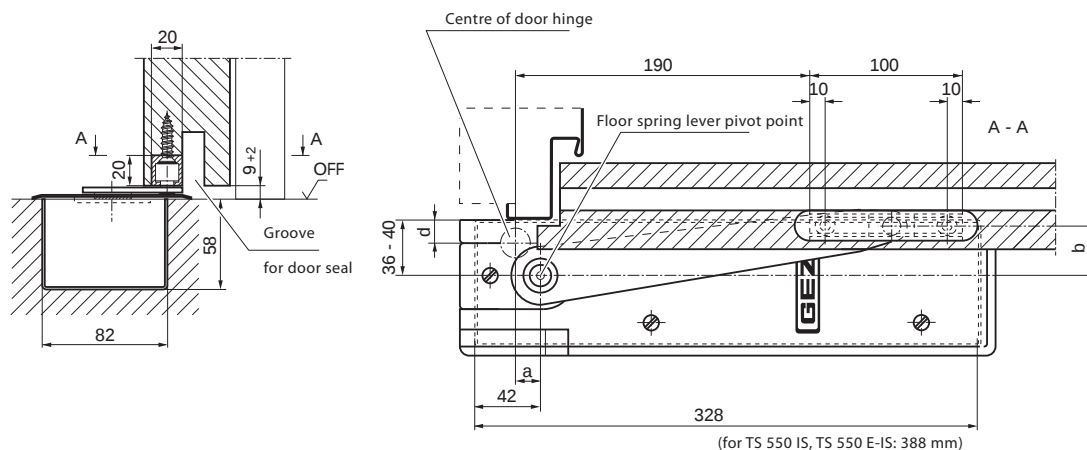
Fig. 34-1 · Installation example: floor spring with lever and guide rail (concealed) to a rebated timber door
