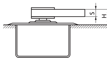
Fig. 32-1 · Guide rail for single action doors
