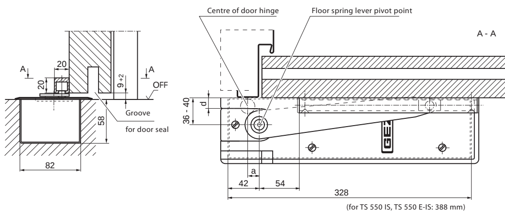
Fig. 33-2 · Installation example: floor spring with lever and guide rail (surface-mounted) to a flush timber door
