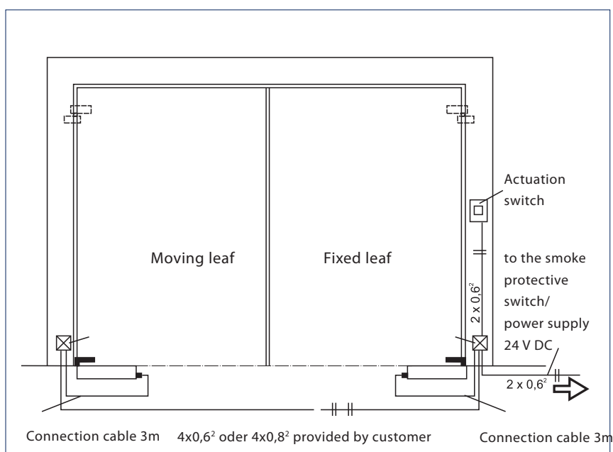
Fig. 35-2 · Electrical installation GEZE TS 550 E-IS / TS 550 E-IS-G
