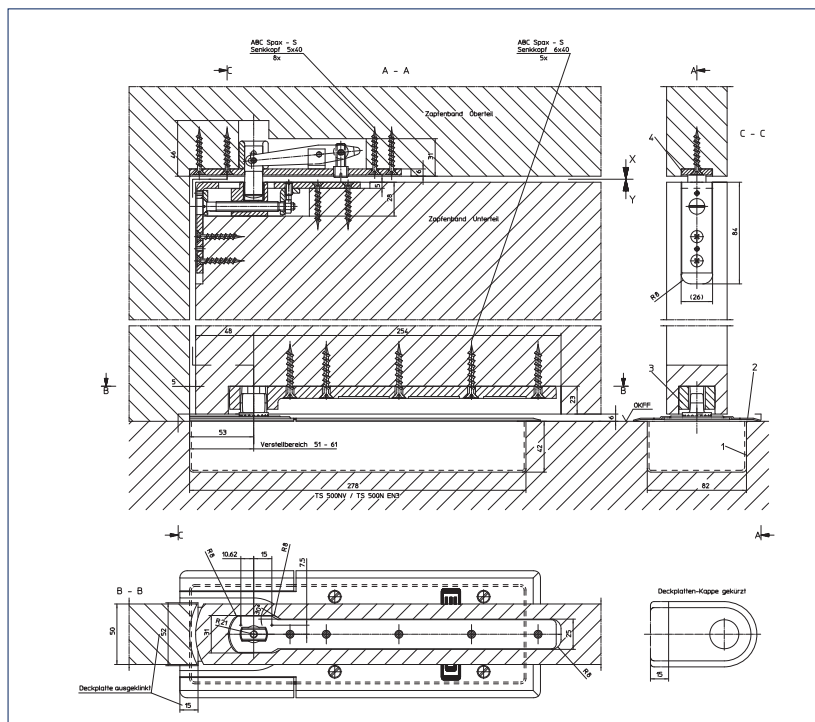
Fig. 30-1 · Standard installation of GEZE TS 500 NV to a double action door
