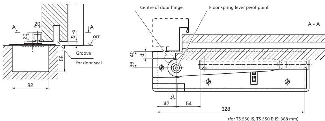
Fig. 33-1 · Installation example: floor spring with lever and guide rail (surface-mounted) to a rebated timber door
