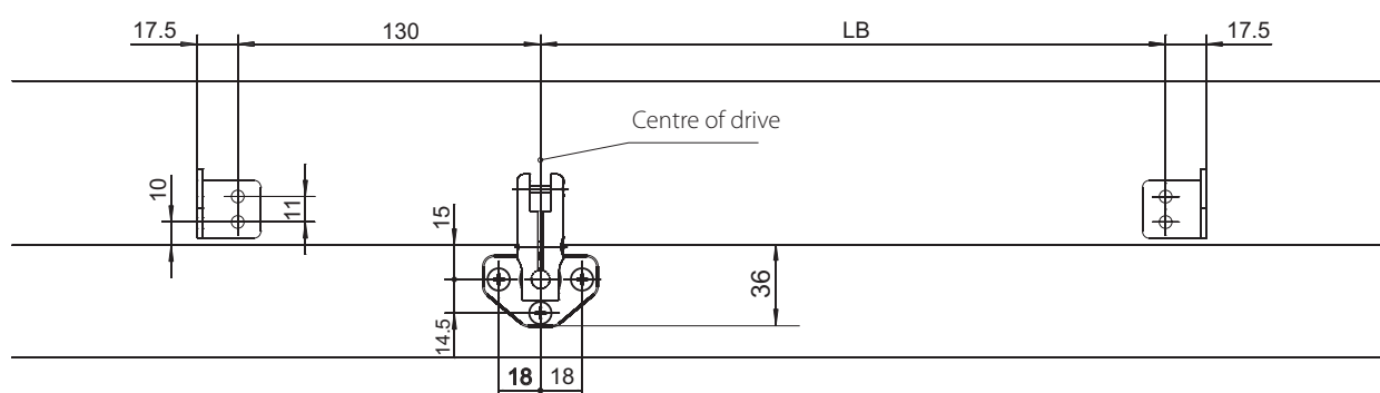
Front view of locking bracket E820/840
