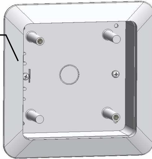
Push Plate Mounting Box (PBS-FM shown)
